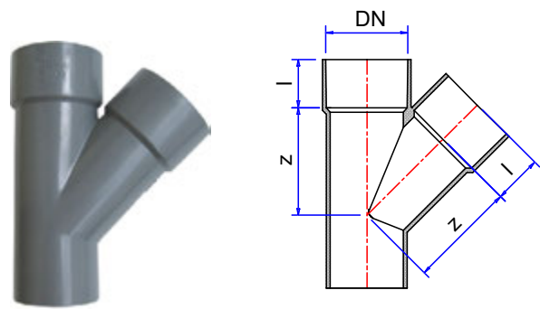
WYE
