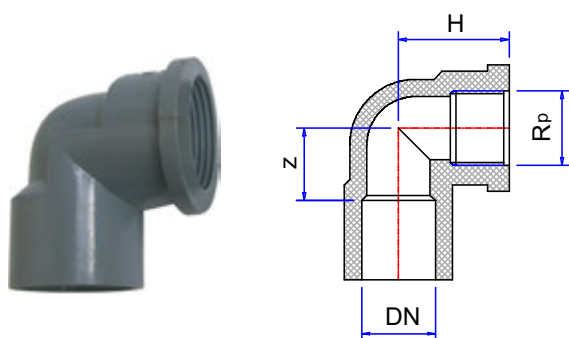
FEMALE ELBOW 90°
