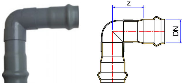
FABRICATED ELBOW 90° WITH GASKET
