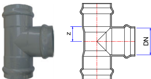
TEE 90° WITH GASKET
