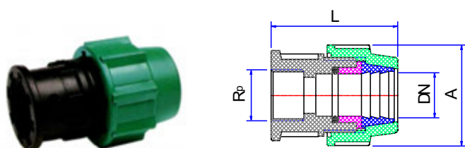
FEMALE ADAPTOR
