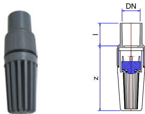
CHECK VALVE
