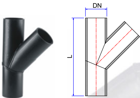
FABRICATED WYE
