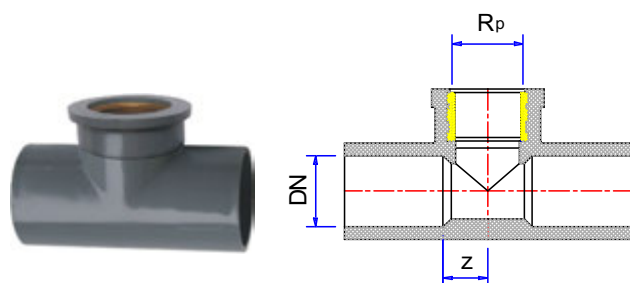
FEMALE TEES 90° WITH BRASS INSERT
