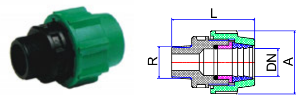
MALE ADAPTOR
