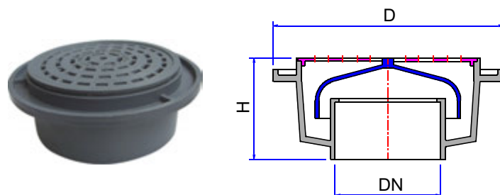
TRAPED FLANGE (ROUND TYPE)
