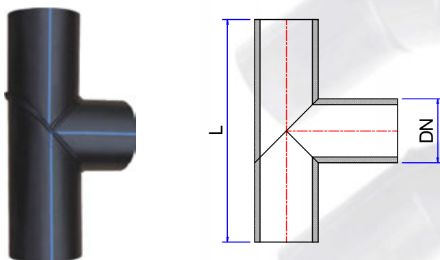
FABRICATED TEE 90°
