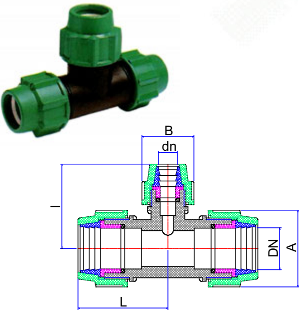
REDUCED TEE 90°
