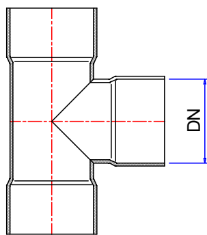
FABRICATED TEE 90°
