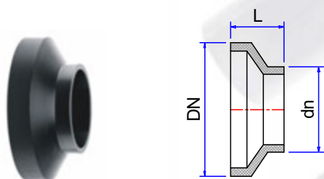
REDUCER CONCENTRIC
