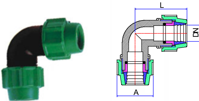
ELBOW 90°
