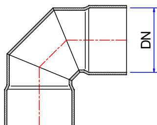
FABRICATED ELBOW 90°
