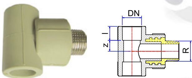
MALE TEE
